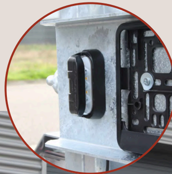
License plate holder with LED lighting
