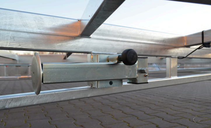
Support legs (4x 1300 kg)
