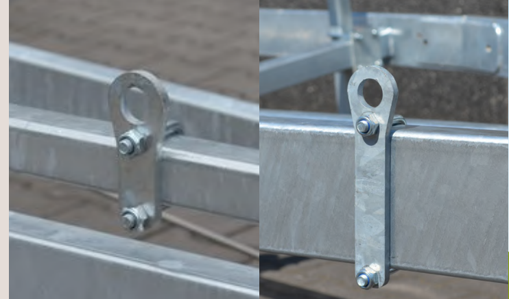
Eyelet for securing tie-down strap
