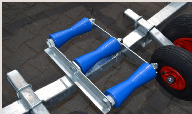
Keel roller tilting system
