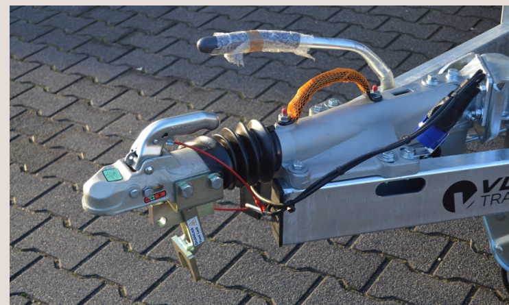
SCM approved lock
