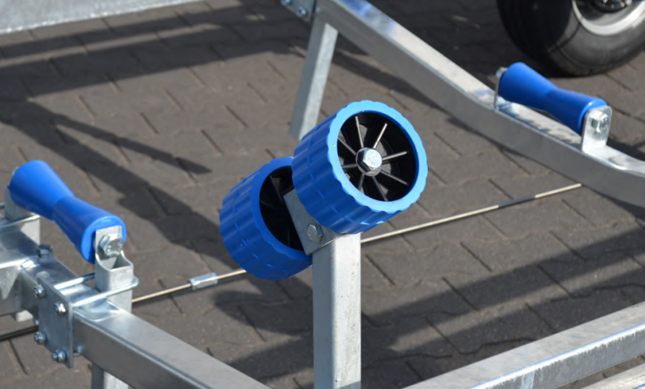
Additional keel rollers
