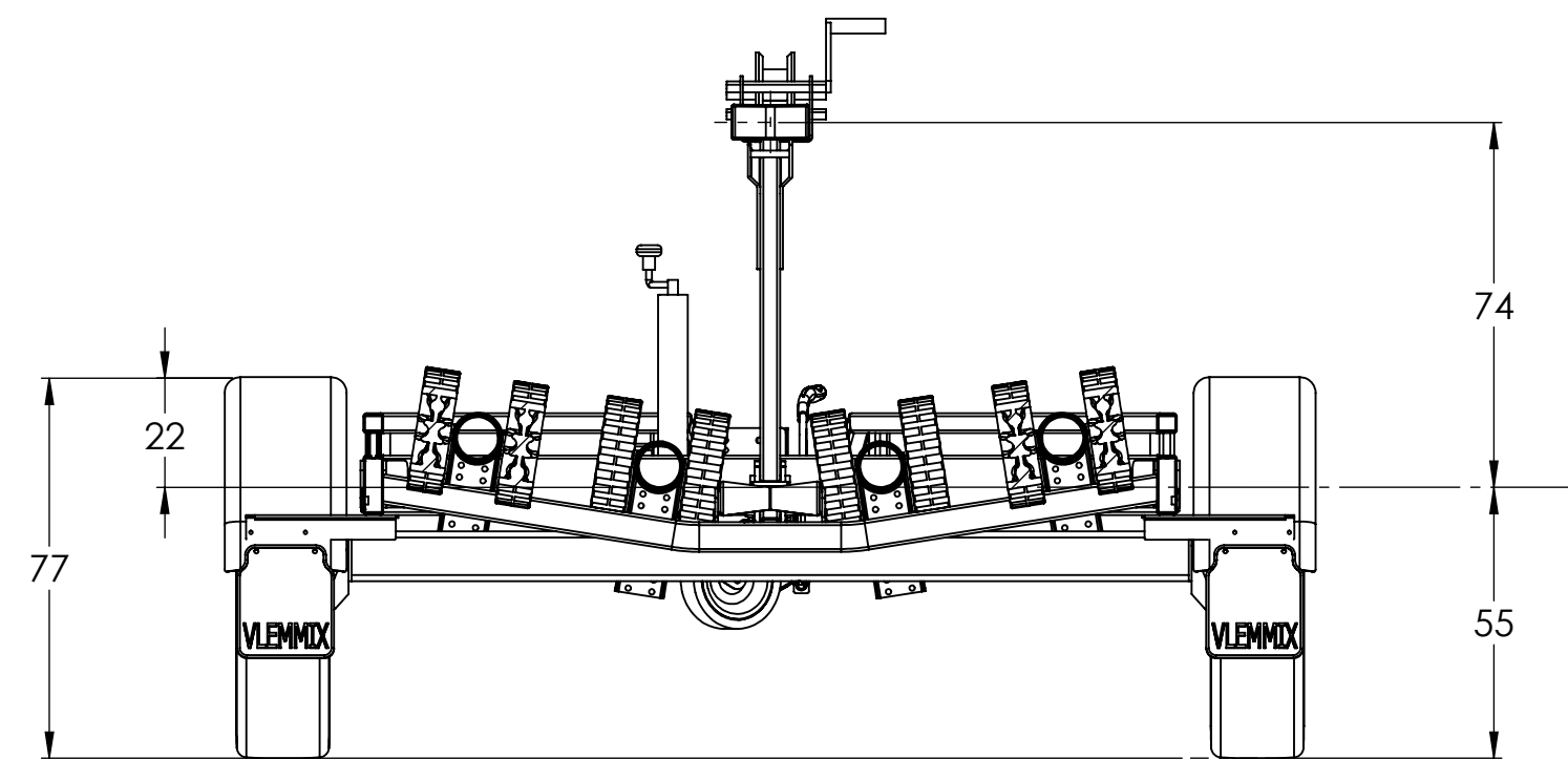
SECTION J-J
