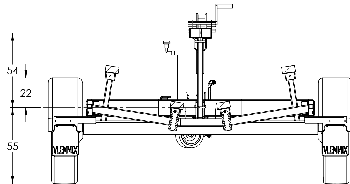
SECTION G-G
