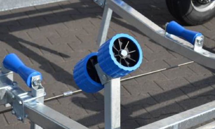
Extra kimrollen
