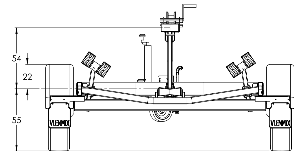
SECTION E-E
